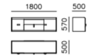
tv base unit SFA-TV 01
