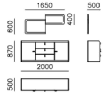
console SFA-CS 01 SFA-CM 01
